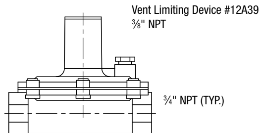
R625P42-0711-11 (2 PSIG Gas System)
